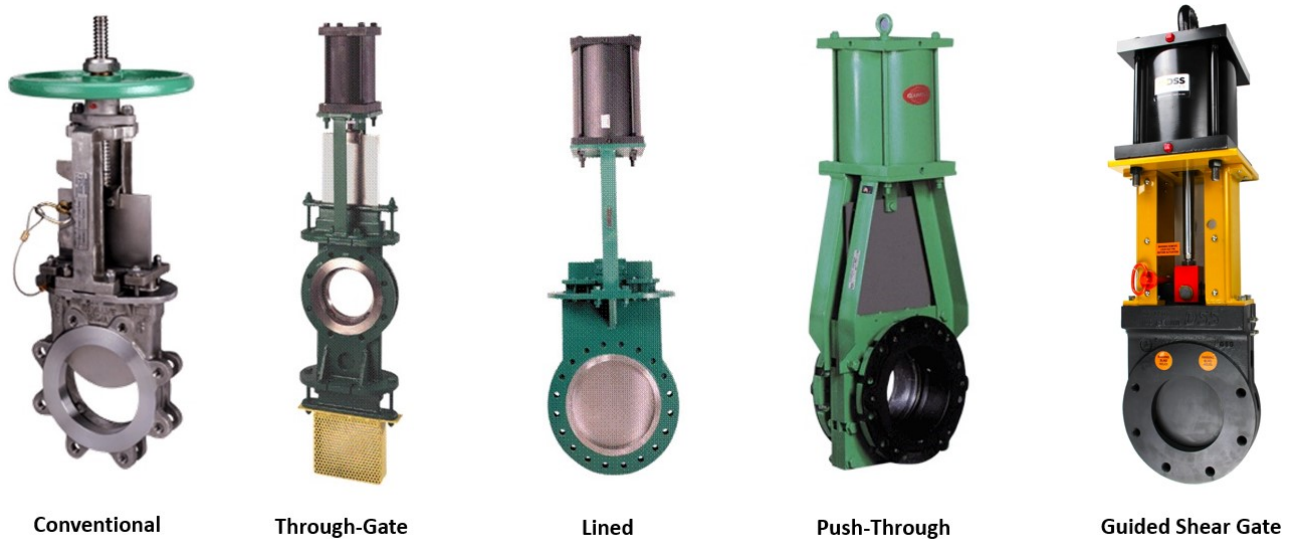
Figure 2 The five types of knife gate valves
